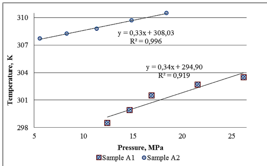
Fig. 3. WAT versus pressure for two live oil samples.
