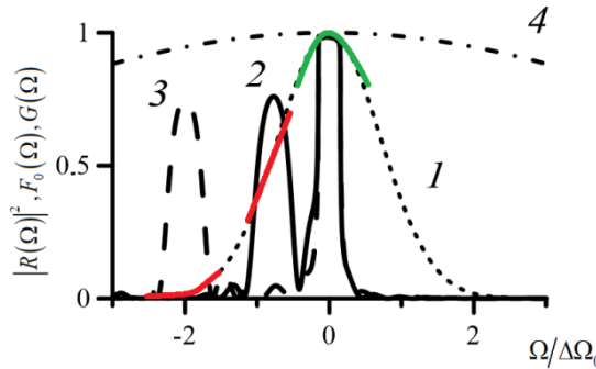
Fig. 4. 1 – incident wave-packet spectrum F_0 of envelop with width, \Delta\Omega_0 = 2/\tau_0 ; 2, 3 – reflection curves for \Delta d/d = 2 \cdot 10^{-5} and \Delta d/d = 5 \cdot 10^{-5} , respectively, d is interplanar spacing for undoped C(400), \Delta d is interplanar spacing difference for the layer and substrate
