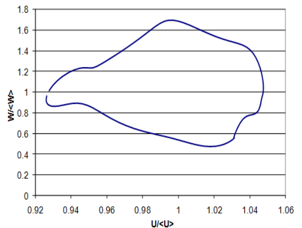
Fig. 4. Normalized dynamic power–voltage characteristics
